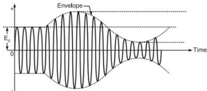
Figure 2. AM under-modulation
