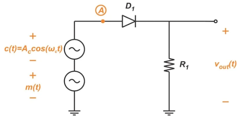
Figure x. Single-diode switching AM Modulator
