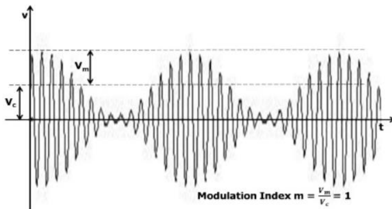
Figure 2. AM critical Modulation
